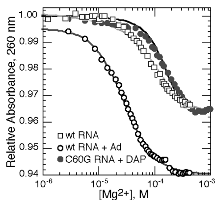
Figure 2. Titration of wild type A-riboswitch (open symbols) or C60G RNA (gray circles) with \text{MgCl}_2 in buffer containing 50 mM \text{K}^+ (20 °C), monitored by absorbance at 260 nm. \text{Mg}^{2+} -dependent baselines have been subtracted from the data sets (see Materials and Methods). Wild type A-riboswitch was titrated in the presence of 82 \mu\text{M} adenine (open circles), or no ligand (open squares); the C60G RNA titration included 82 \mu\text{M} DAP (gray circles). Titration of the wild type RNA with ligand has been fit to the Hill equation (midpoint 29.0 \mu\text{M} \text{Mg}^{2+} , n = 1.58 ). The other two curves are optimum fits of a \text{Mg}^{2+} -dependent two-state equilibrium between E and \text{I}_{\text{dock}} forms (wild type RNA) or E and \text{I}_{\text{LBP}} forms (C60G RNA) (see Results for further explanation).
