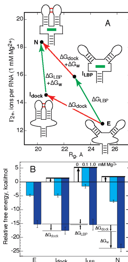
Figure 6. Effects of \text{Mg}^{2+} on the A-riboswitch folding landscape. (A) Four states of the A-riboswitch, distinguished by their dimensions ( R_g ) and excess \text{Mg}^{2+} ( \Gamma_{2+} , reported at 1 mM \text{Mg}^{2+} ). See Discussion for definitions of the four states. Arrows connecting the RNA forms define a thermodynamic cycle with three free energies, all of which are potentially \text{Mg}^{2+} -dependent. The number of ions taken up ( \Delta\Gamma_{2+} ) in the reaction defined by each arrow is indicated. (B) Stabilities of each of the RNA forms from panel A, relative to the extended form (E) in its standard state (50 mM \text{K}^+ buffer without \text{Mg}^{2+} ). Stabilities of the ligand-bound RNA forms (N and I_{\text{LBP}} ) are calculated for an adenine concentration of 10 \mu\text{M} . Thick arrows, free energies of the two-state equilibria between E and each of the three other forms; cyan and blue bars, stabilization of each form by 0.1 or 1.0 mM bulk \text{Mg}^{2+} concentration, respectively. Calculations of the three \Delta G values defined in panel A are illustrated for 1 mM \text{Mg}^{2+} (arrows labeled by \Delta G ). Error bars for the N and E state \text{Mg}^{2+} –RNA interaction free energies are based on the reproducibility of the \Gamma_{2+} data that were integrated to find \Delta G_{\text{RNA-2+}} (Figure 5); errors for the other two forms include an additional estimated uncertainty from the method used to interpolate the free energies.
