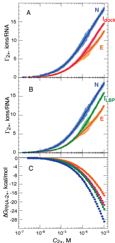
Figure 5. Excess \text{Mg}^{2+} ( \Gamma_{2+} ) as a function of bulk \text{Mg}^{2+} concentration ( C_{2+} ) for wild type and C60G RNAs in standard conditions (50 mM \text{K}^+ , 20 °C), with and without the ligand DAP present (250 \mu\text{M} ). Six or seven independent data sets were merged to obtain each titration curve; errors are shown in the plots as lighter color bars (see Materials and Methods). (A) Wild type RNA in the presence (blue) or absence (magenta) of ligand. C60G RNA in the absence of ligand is shown for comparison (orange). (B) C60G RNA in the presence (green) or absence (orange) of ligand. Wild type RNA in the presence of ligand is shown for comparison (blue). (C) Free energies of \text{Mg}^{2+} –RNA interaction ( \Delta G_{\text{RNA-}2+} ) calculated from \Gamma_{2+} curves in panels A and B (see Materials and Methods). Blue, native RNA (N); orange, C60G RNA in the absence of ligand (E); green, the I_{\text{dock}} conformation, extrapolated from wild type RNA at 1 mM \text{Mg}^{2+} ; magenta, I_{\text{LBP}} conformation, extrapolated from C60G RNA bound to ligand at 1 mM \text{Mg}^{2+} .
