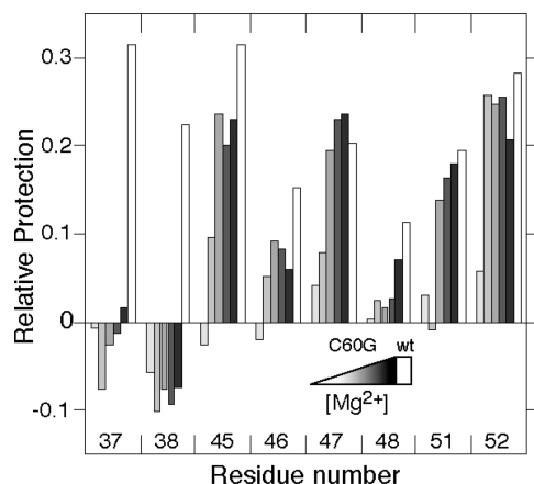
Figure 4. Hydroxyl radical footprinting results for the wild-type and C60G variant A-riboswitch (data analysis was as described in Materials and Methods). Experiments were performed in standard buffer at 0 °C, with the indicated amount of \text{Mg}^{2+} and 250 \mu\text{M} DAP present in all but the unfolded control samples. The difference in normalized reactivity between the control unfolded form (RNA in the absence of \text{Mg}^{2+} and DAP) and the sample RNA (with DAP and \text{Mg}^{2+} ) is plotted; a positive number represents reduced reactivity in the sample RNA. Open column, wild type RNA with 5 mM \text{Mg}^{2+} ; gray – black columns, C60G RNA with increasing \text{Mg}^{2+} concentrations of 0.1, 0.2, 0.5, 1.0, and 5.0 mM. Residue numbering is the same as Figure 1A. Relative reactivities of nucleotides 32–75 are in Supporting Information (Figure S2).
