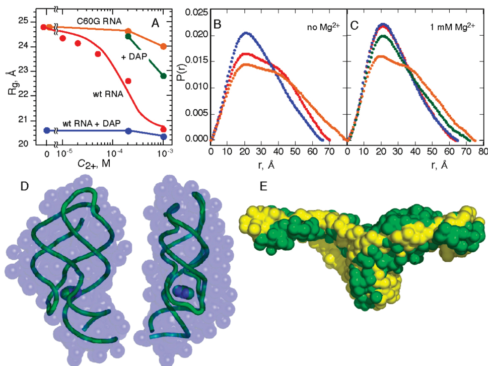
Figure 3. SAXS studies of wild type and variant A-riboswitch RNAs in standard buffer; ligand is 250 \mu M DAP, where present. Samples were equilibrated with the indicated bulk \text{Mg}^{2+} concentrations ( C_{2+} ). (A) R_g as a function of bulk \text{Mg}^{2+} concentration for wild type RNA with (blue) or without (red) ligand, or C60G RNA with (green) or without (orange) ligand. The solid red line is the best fit of a \text{Mg}^{2+} -dependent two-state equilibrium between E and I_{\text{dock}} forms of the RNA (see text). (B) Distance distribution function P(r) for RNAs in the absence of \text{Mg}^{2+} : wild type RNA with (blue) or without (red) ligand, or C60G RNA without ligand (orange). (C) P(r) for RNAs with 1 mM bulk \text{Mg}^{2+} concentration: wild type RNA with (blue) or without (red) ligand, and C60G RNA with (green) or without (orange) ligand. (D) Reconstruction from SAXS data of the wild type A-riboswitch bound to ligand in the presence of \text{Mg}^{2+} . The RNA backbone from the corresponding crystal structure (1Y26) has been aligned with the calculated density; the bound adenine ligand is shown as a space-filling model. The two views differ by 90° rotation. (E) Reconstruction from SAXS data of the C60G (green) and G38C (yellow) RNAs in the absence of ligand or \text{Mg}^{2+} . The two structures are superimposed to show their similar overall shape.
